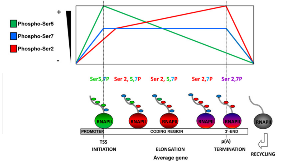
Figure 3. RNAPII CTD phosphorylation profile in Sacharomyces cerevisiae . During transcription initiation and promoter escape RNAPII CTD is phosphorylated on Ser5 (Ser5P) [48, 78]. Concurrently, Ser7 is phosphorylated (Ser7P), establishing a bivalent mark at both protein-coding and noncoding genes [74-76]. Shortly after promoter dissociation, Ser5P is rapidly removed while phosphorylated Ser2 (Ser2P) and Ser7P continue to accumulate [70, 77]. Finally, all CTD marks are rapidly removed at the end of transcription, and the hypophosphorylated RNAPII (in grey) is ready to assemble into the pre-initiation complex and re-initiate transcription [73, 79-80]. Small circles represent phosphorylated serine residues (green circles for Ser5P, blue circles for Ser7P and red circles for Ser2P). Differently colored big circles represent the distinct phosphorylated forms of RNAPII during initiation, elongation and termination. TSS: transcription start site; p(A): polyadenylation site.
