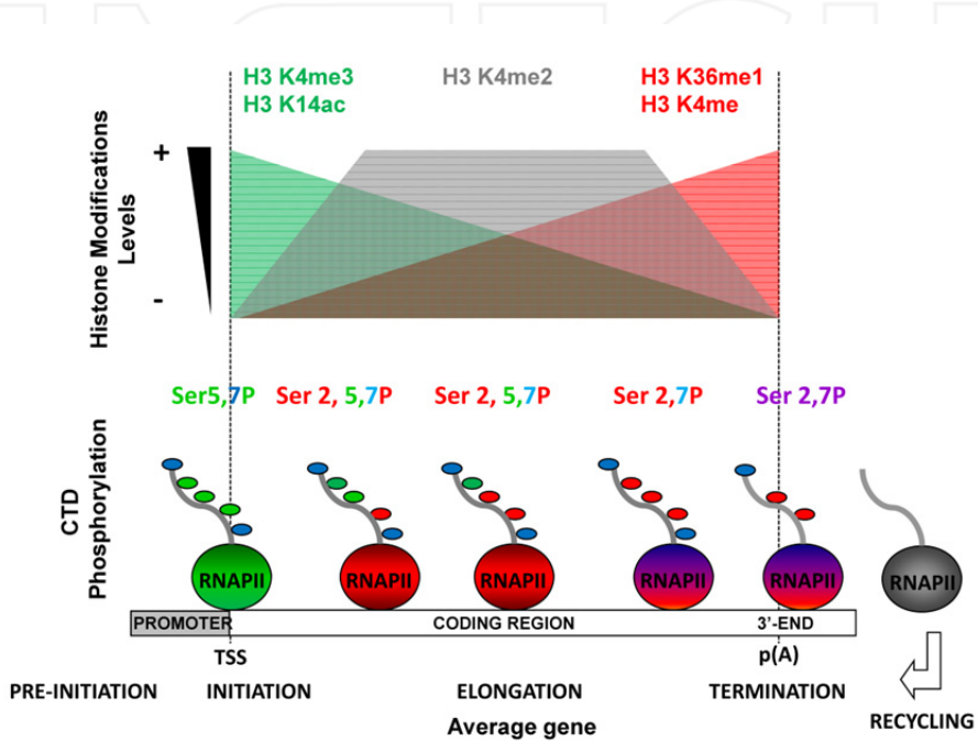
Figure 6. Histone H3 tri-, di-, and mono-methylation and acetylation during RNAPII transcription in S. cerevisiae .
